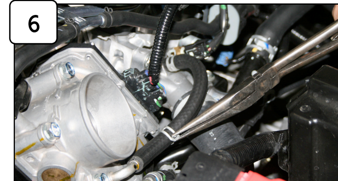
6 Replace throttle body coolant line with 5/16" hose provided and secure with clamps used from step 5.
