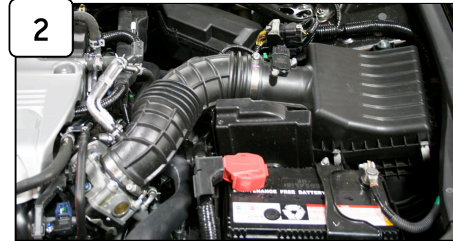
2 Complete Stock intake. Please disconnect battery terminals before installation. Do not attempt to install kit if vehicle is not cold!
