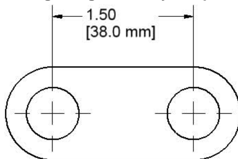
DRILLING TEMPLATE
