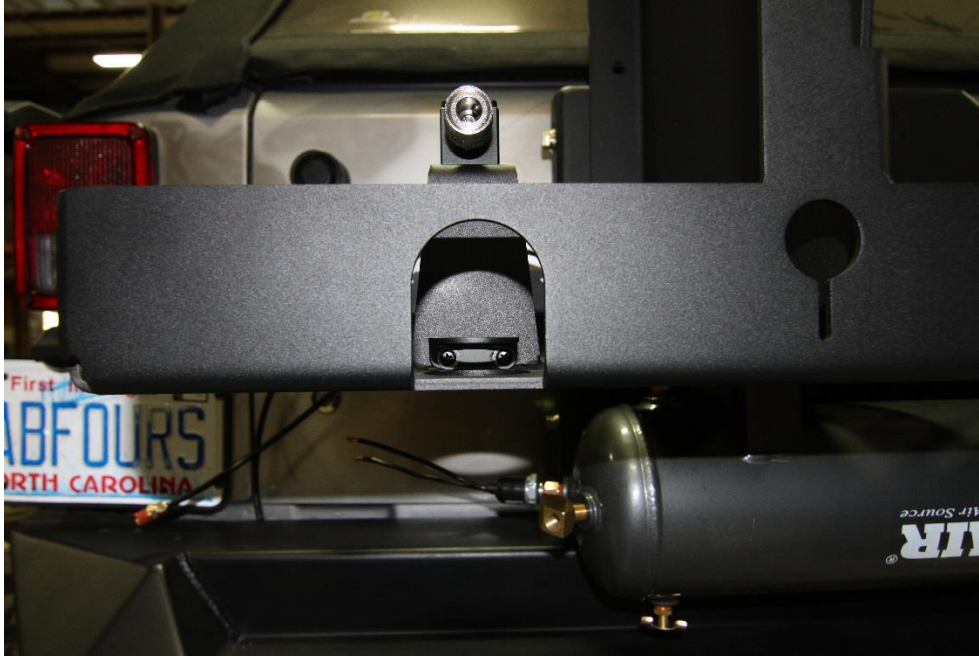
Figure 3: Pressure Gauge Bracket and 6-Port Block
