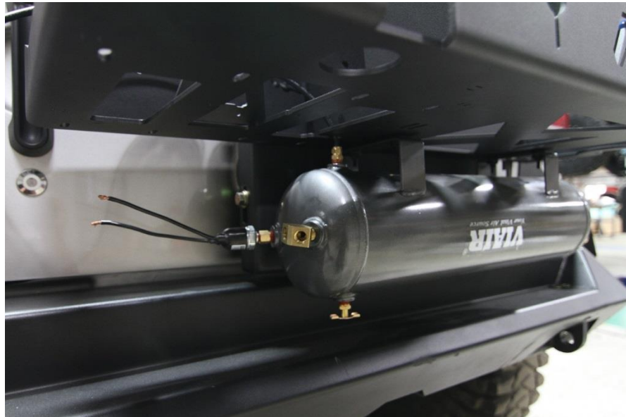
Figure 2: Pressure Switch, Y Fitting, 1/4" NPT Outlet, and Drain Cock
