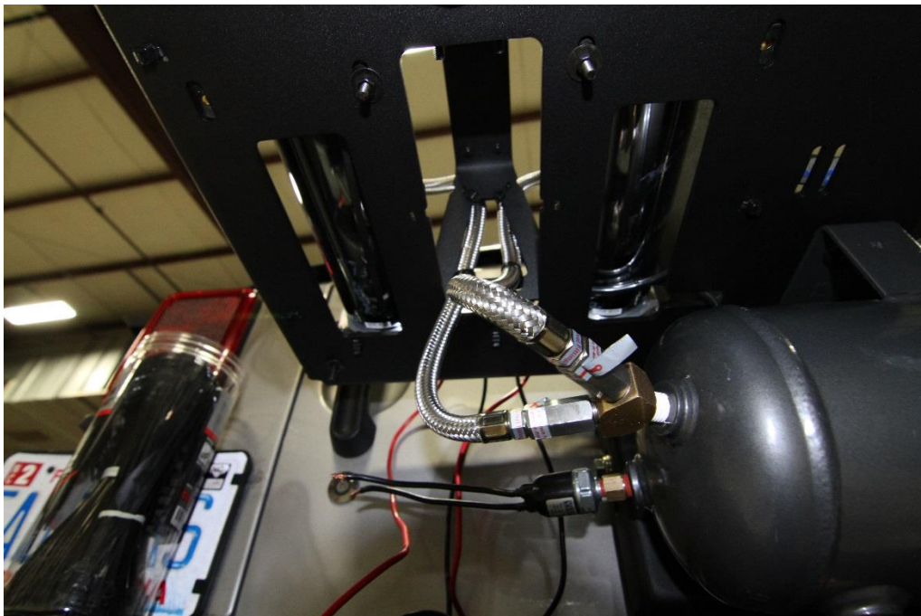
Figure 6: Line Routing From Compressors
