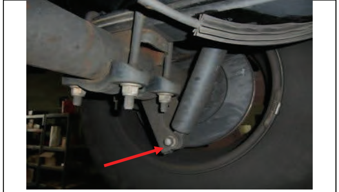
Work on one side at a time and remove lower shock bolt
