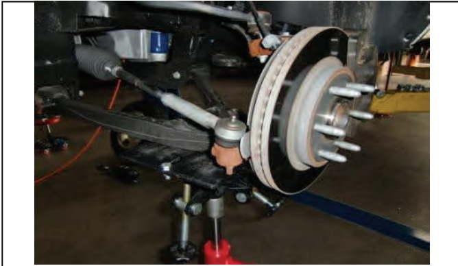
Support suspension with jack
