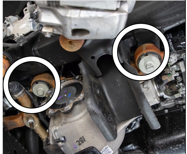
Figure 23: Driver Side Differential Mounting
