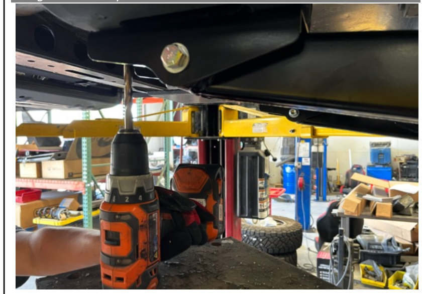
Figure 69: Compression Strut Bracket with Frame Crossmember
