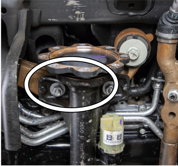
Figure 22: Passenger Side Differential Mounting
