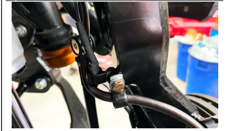
Figure 64: Passenger Side: Middle Spindle Tab and P-clamps
