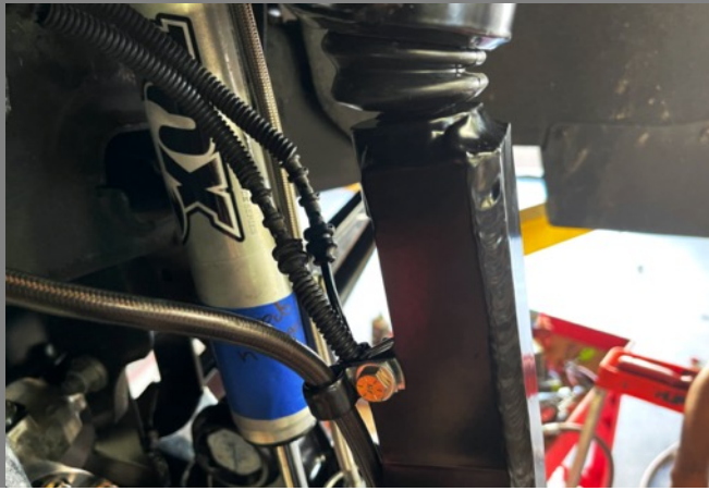
Figure 65: Driver Side Top Spindle Tab & P-clamps
