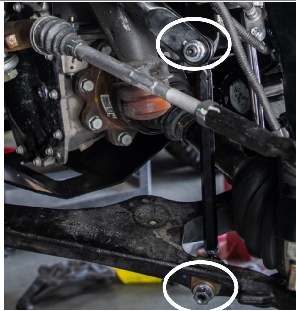
Figure 67: Sway Bar End Links
