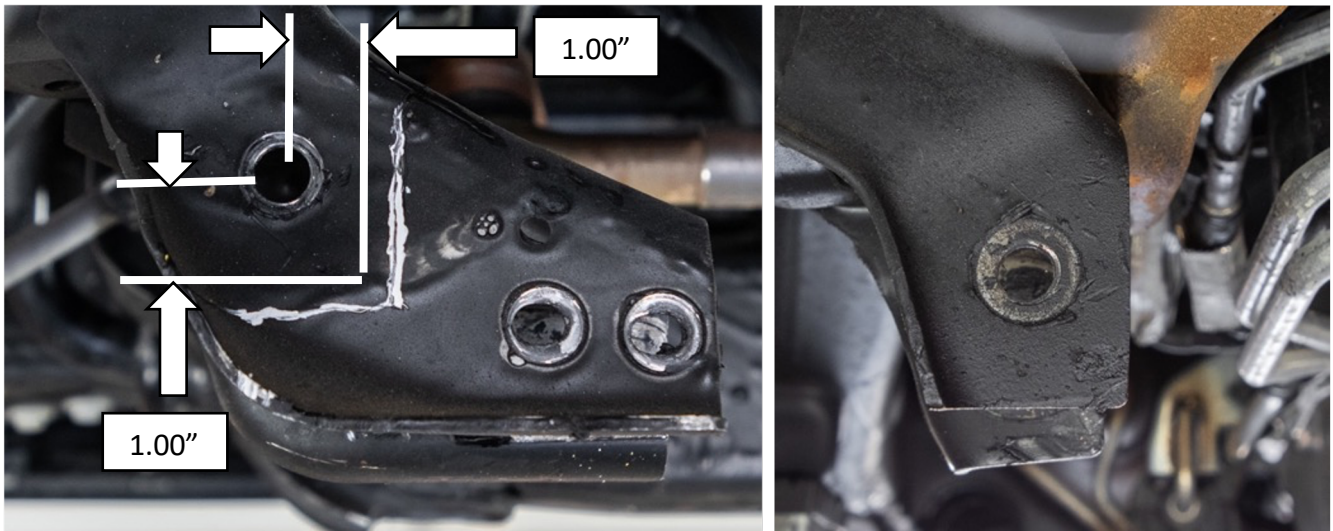
Figure 26: Trim Rear Crossmember
