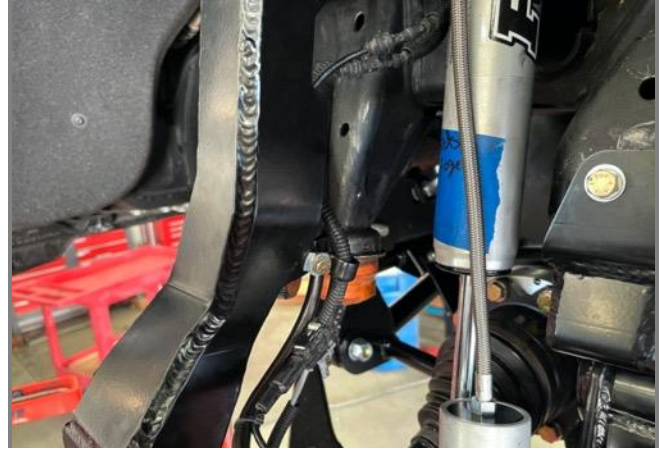
Figure 66: Driver Side Middle Spindle Tab & P-clamps
